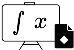
Mathematical Research
