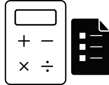
Menial Computation
