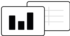
Knowledge Work
