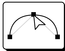
SVG Competition
